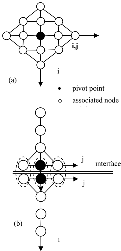
Fig. 3 Representative of the (a) stencil for the governing equations for the inner nodes of the material (b) stencil for the displacement component, u_x , at the interface of the bilayer composite.
