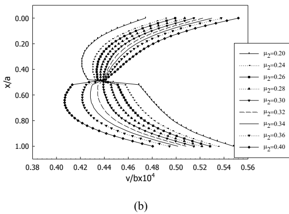
Fig. 5 (a) Variation of normalized displacement component (u/a) and (b) Variation of normalized displacement component (v/b) for different Poisson's ratios of lower material at y/b=0.24 of the bilayer composite.
