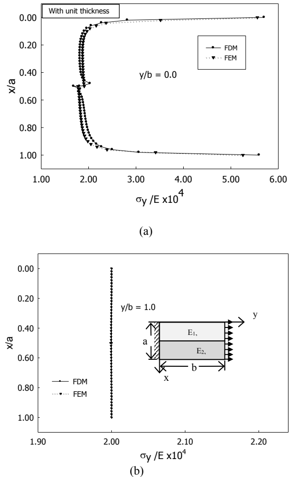
Fig. 4 Comparison between FEM vs FDM approach: normalized normal stress ( \sigma_y/E ) distribution at (a) y/b = 0.0 , (b) y/b = 1 . Please note: for top layer, E = E_1 , and for bottom layer, E = E_2 .
