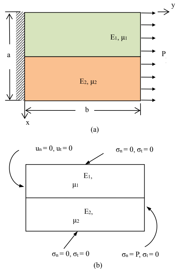
Fig. 1 (a) A schematic diagram of a bilayer composite subjected to axial loading, (b) the corresponding boundary conditions where, \psi is the displacement potential function. Eq. (1) is valid for both plane stress and plane strain conditions.
