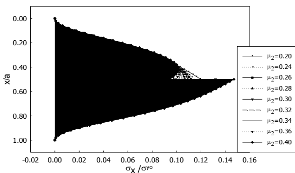
Fig. 6 Variation of normalized normal stress ( \sigma_x / \sigma_y^0 ) for different Poisson's ratios of lower material at y/b=0.24 of the bilayer composite.
